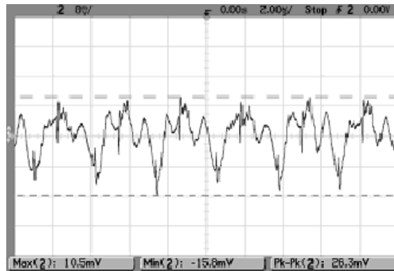
Fig. 53 Typical output ripple voltage of AVO75-48S2V5 room temperature, I_o=I_{o,max}
