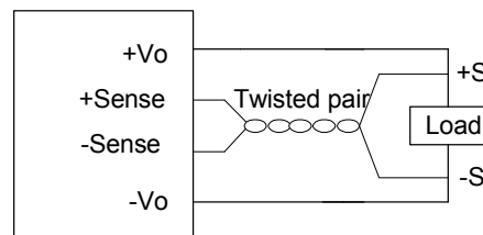
Fig. 72 Sense connections
