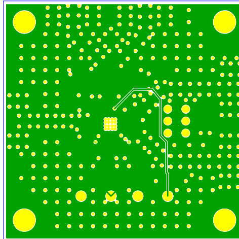
Figure 52. Evaluation Board Power Plane, Internal Layer 2
