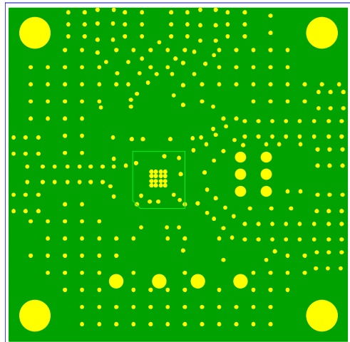
Figure 51. Evaluation Board Ground Plane, Internal Layer 1
