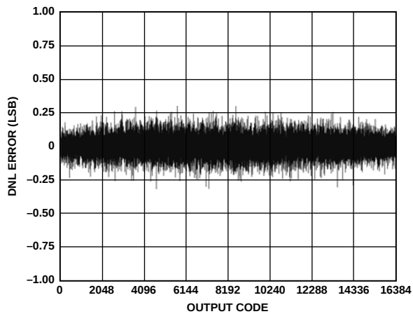
Figure 37. DNL Error vs. Output Code, 80 MSPS, A_{IN} = 15 MHz
