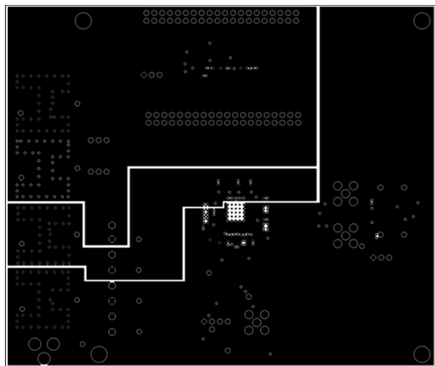
Figure 55. LVDS Mode Evaluation Board Layout, Power Plane 1
