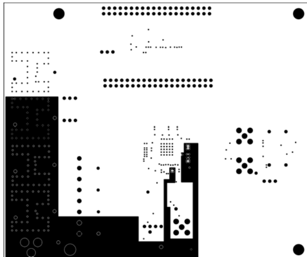
Figure 56. LVDS Mode Evaluation Board Layout, Power Plane 2
