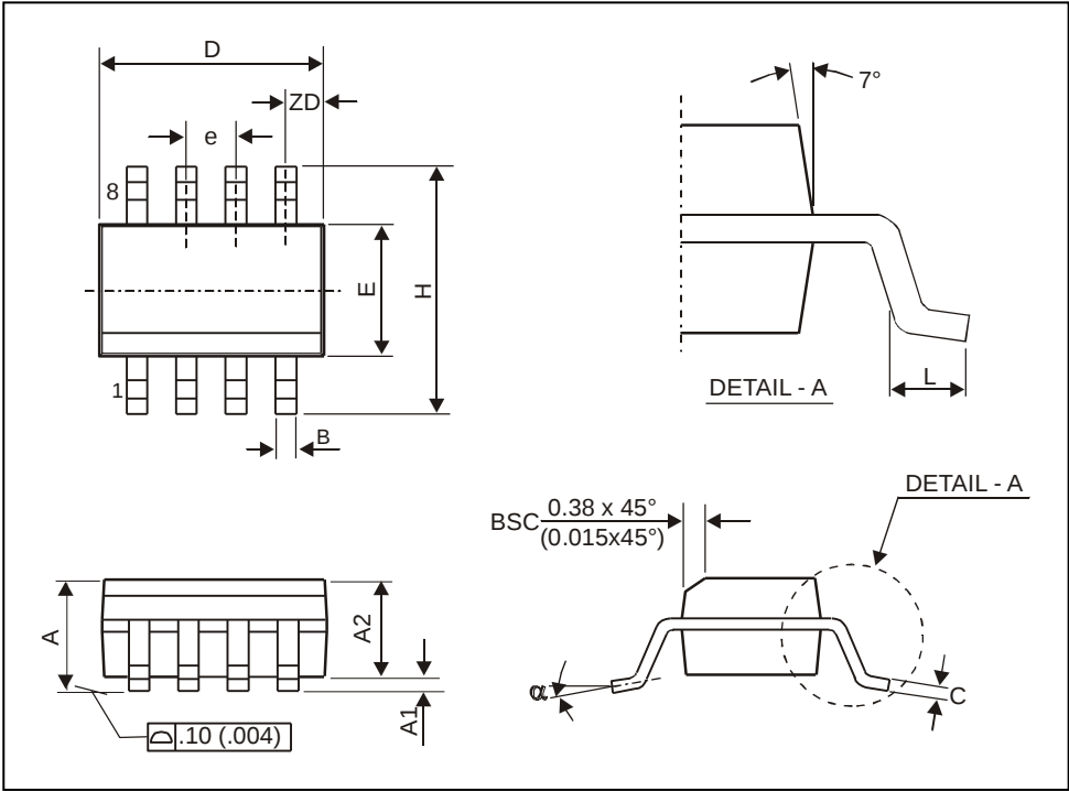
Fig. 13: SOIC8 (Small Outline Integrated Circuit)
