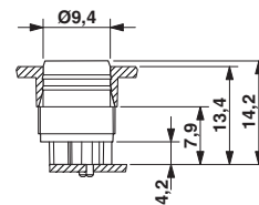
Dimensioned drawing
