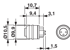
Dimensioned drawing
