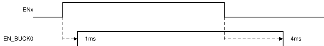
Figure 9. Typical Start-Up and Shutdown Sequencing
