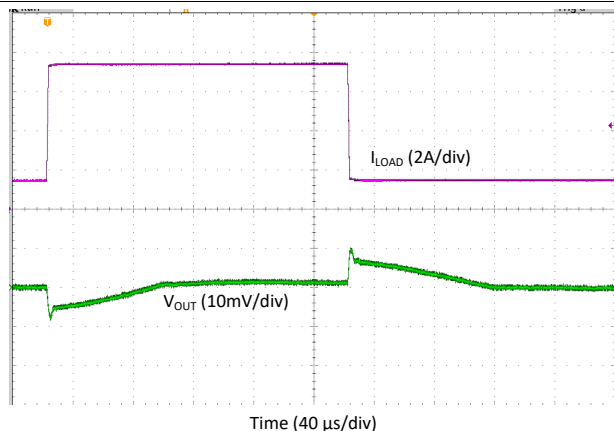
Figure 34. Transient Load Step Response, Forced-PWM-Four-Phase Mode, T_A = +25^\circ\text{C}
