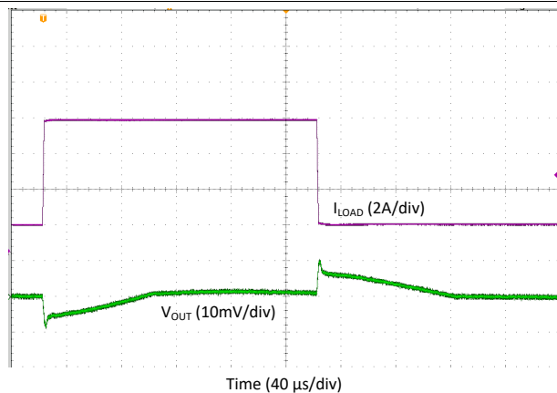
Figure 35. Transient Load Step Response, Forced-PWM-Four-Phase Mode, T_A = -40^\circ\text{C}
