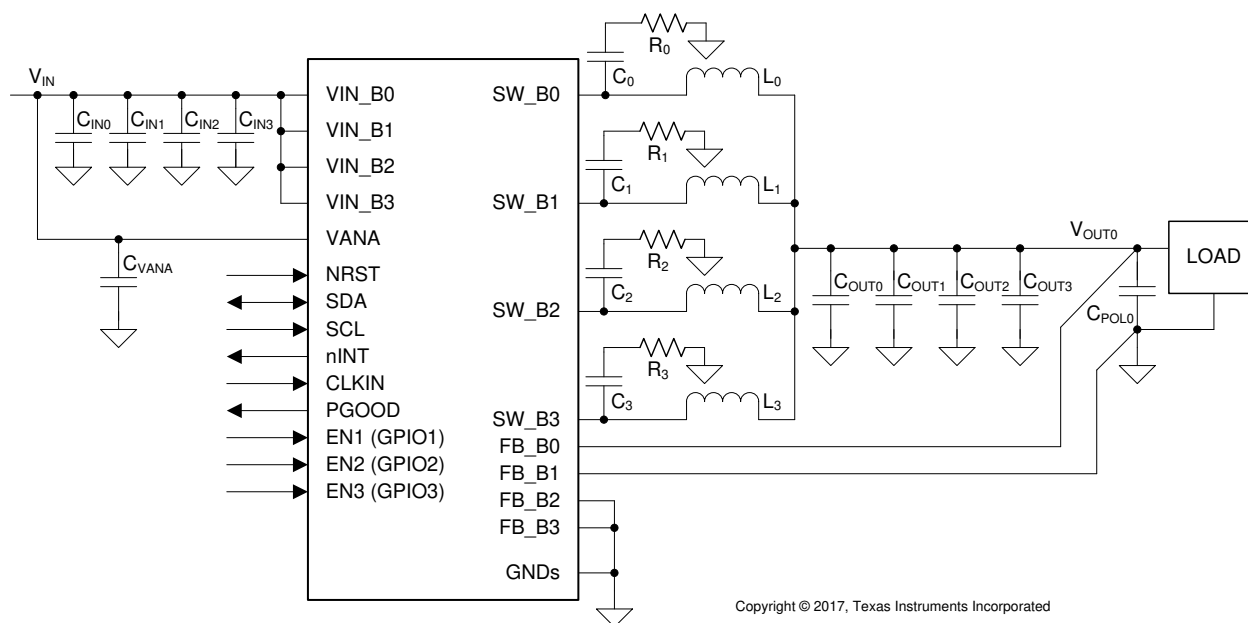
Figure 21. 4-Phase Configuration
