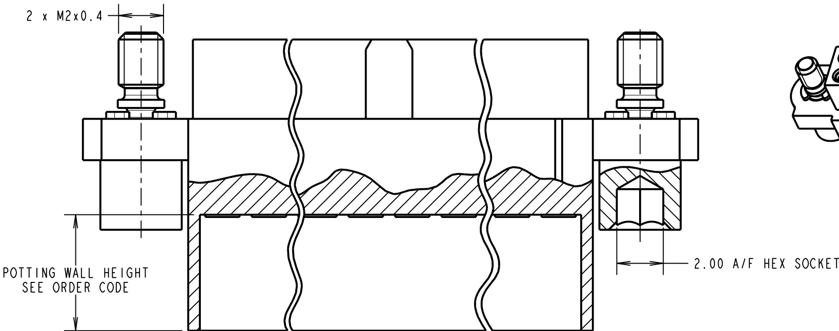
PART SECTION Y-Y
