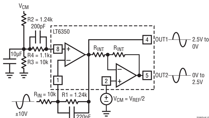
Figure 7. LT6350 Converting a \pm 10 V Single-Ended Signal to a \pm 2.5 V Differential Input Signal
