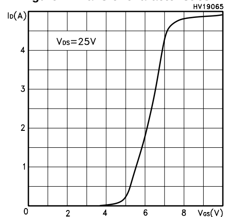
Figure 7: Transfer characteristics
