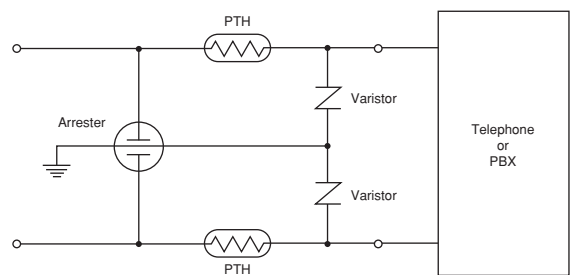
(5) Telecommunication Circuit
