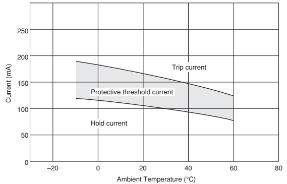
PTGL07AR560M9A51B0
