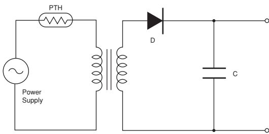
(1) Transformer Protection Circuit 1
