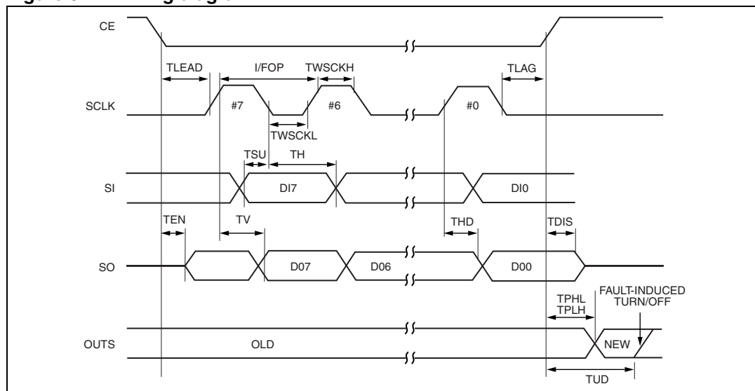
Figure 5. Timing diagram.
