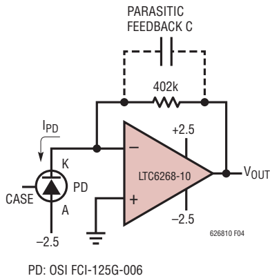
Figure 4. LTC6268-10 and Low Capacitance Photodiode in a 402k \Omega TIA
