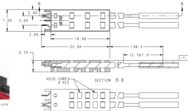
2 position mini hermaphroditic wire to board lead assembly
