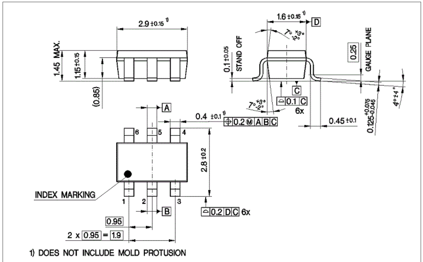
Figure 5 Package Drawings
