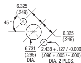
PANEL LAYOUT
