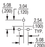
PCB LAYOUT
