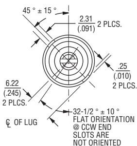
Shaft End Detail 3862
