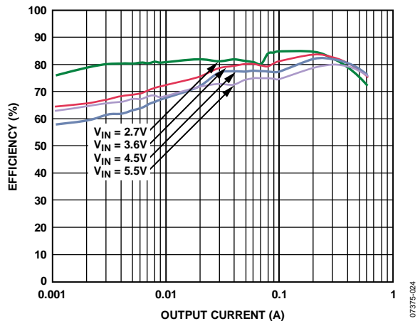
Figure 14. Efficiency, V_{OUT} = 1.0 V
