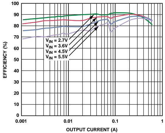
Figure 13. Efficiency, V_{OUT} = 1.8 V
