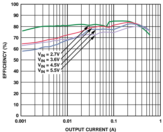
Figure 14. Efficiency, V_{OUT} = 1.0\text{ V}
