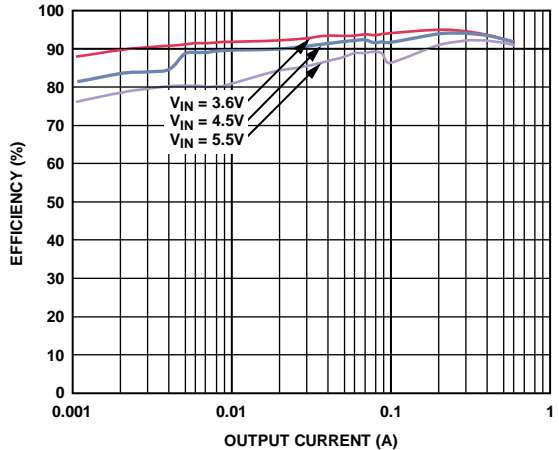
Figure 15. Efficiency, V_{OUT} = 3.3\text{ V}
