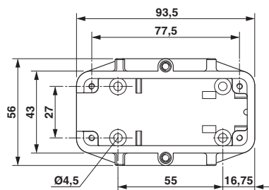
Dimensional drawing top view
