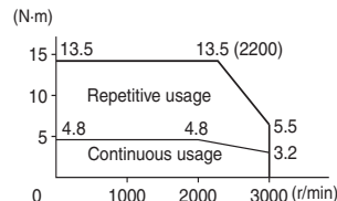
R88M-G1K020T (1 kW)
