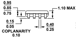
Figure 45. 8-Lead Mini Small Outline Package [MSOP] (RM-8) Dimensions shown in millimeters
