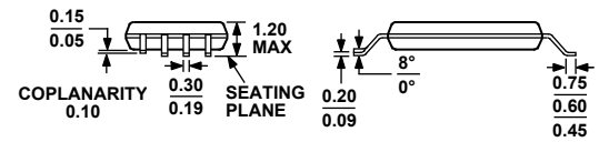
Figure 46. 8-Lead Thin Shrink Small Outline Package [TSSOP] (RU-8) Dimensions shown in millimeters
