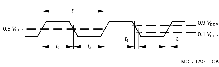
Figure 14 Test Clock Timing (TCK)
