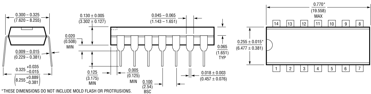
N Package 14-Lead PDIP (Narrow 0.300) (LTC DWG # 05-08-1510)
