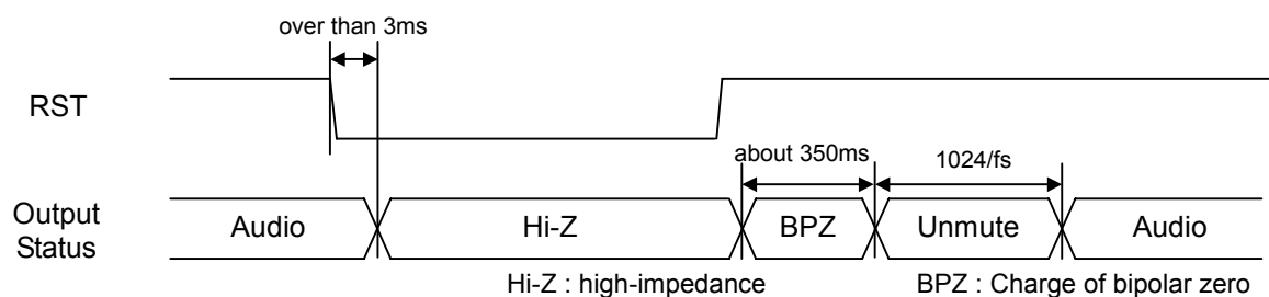
Figure 1. Reset Timing
