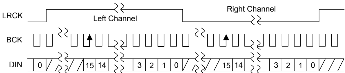
Figure 3.3. 16 bits LSB Justified Data Format
