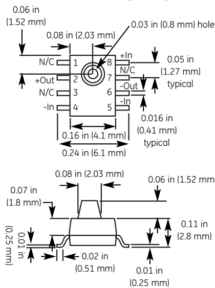
NPP-301 Series package diagram
