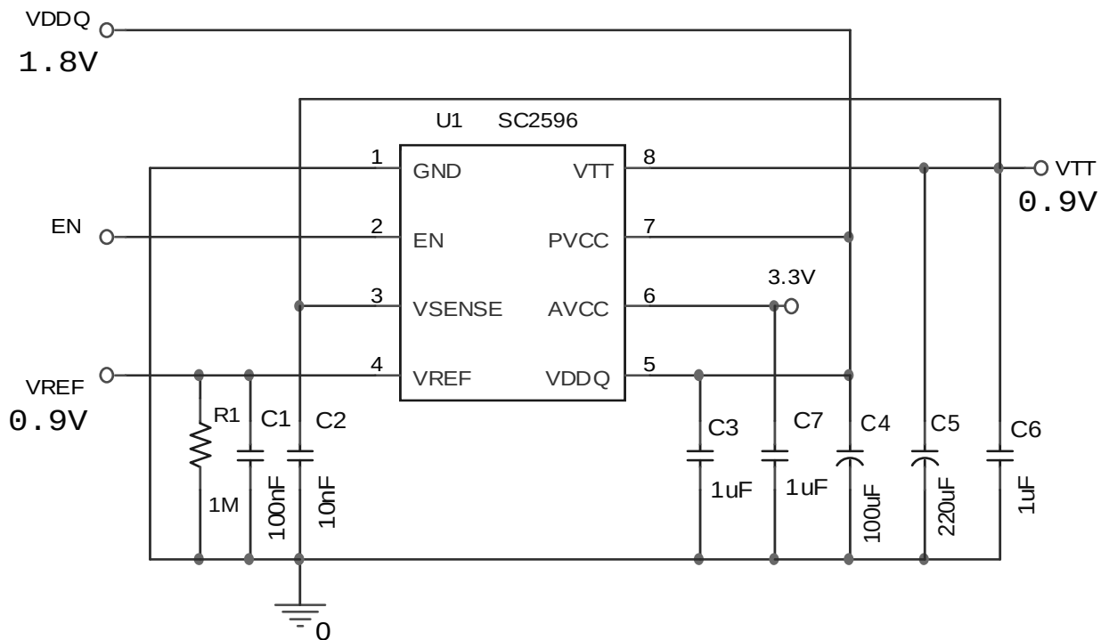
DDR-II VTT Solution
