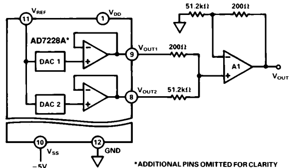
Figure 11. Coarse/Fine Adjust Circuit
