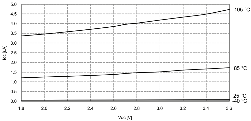
Figure 37-268. Power-down mode supply current vs. V_{CC} . All functions disabled
