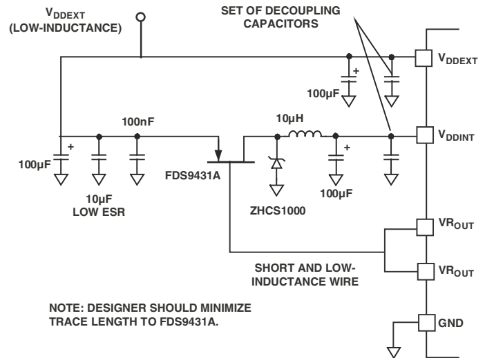
Figure 6. Voltage Regulator Circuit
