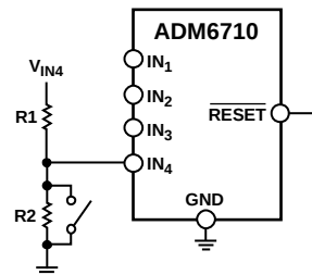
Figure 15. Addition of Manual Reset ( IN_4 is an Adjustable Input)
