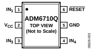
Figure 3. ADM6710Q Pin Configuration
