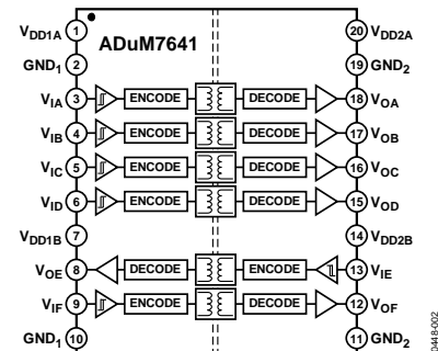
Figure 2. ADuM7641
