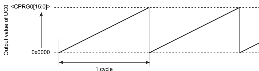
Figure 12-6 Cycle of rectangular wave in PPG mode
