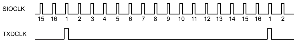
Figure 13-7 Generation of Transmission Clock in UART mode
