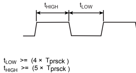
Figure 14-6 SCLK Input
