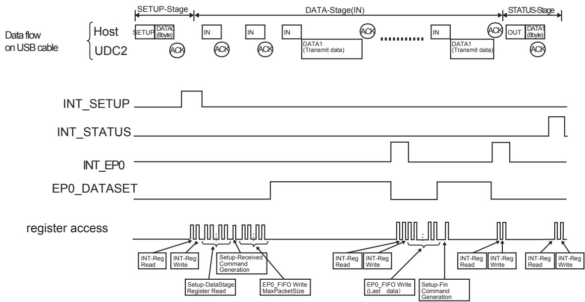
Figure 16-22 Flow of the control in Control-RD transfer
