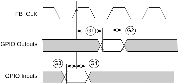
Figure 26. GPIO Timing
