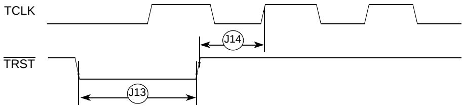
Figure 30. \overline{\text{TRST}} Timing
