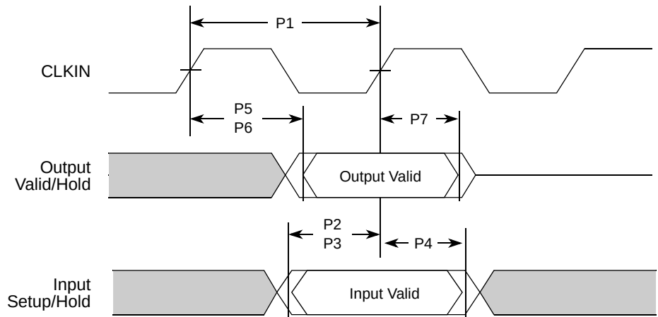
Figure 13. PCI Timing
