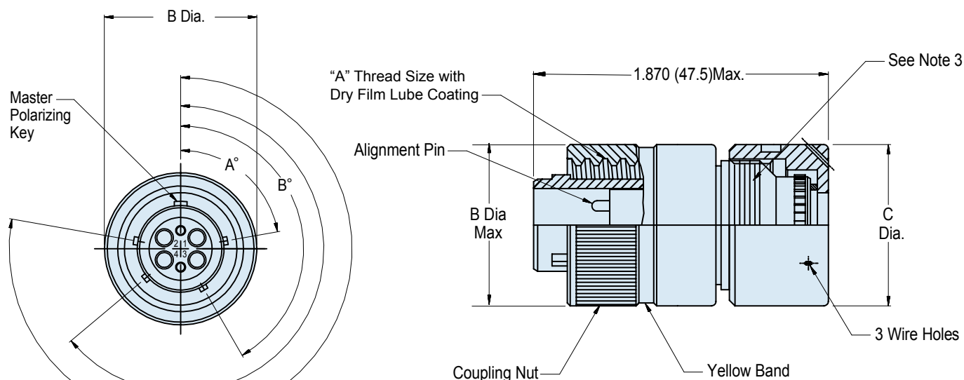
06 - PLUG WITHOUT STRAIGHT BACKSHELL
