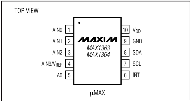
Pin Configuration
