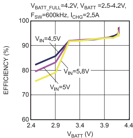
Constant Current Charge Efficiency V_{BATT\_FULL}=4.2V , V_{BATT}=2.5-4.2V , F_{SW}=600kHz , I_{CHG}=2.5A
