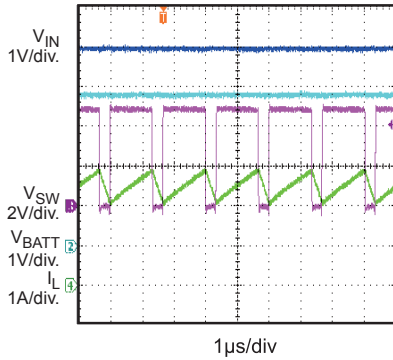
CC Charge Steady State V_{BATT\_FULL}=4.2V , V_{BATT}=3.7V , F_{SW}=600kHz
