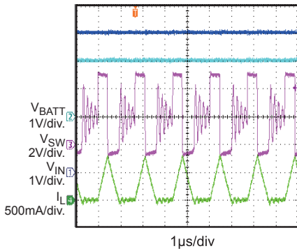
TC Charge Steady State V_{BATT\_FULL}=4.2V , V_{BATT}=2V , F_{SW}=600kHz
