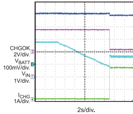
Auto Recharge V_{BATT\_FULL}=4.2V
