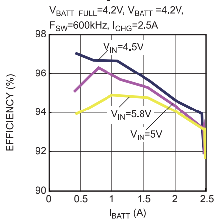
Constant Voltage Charge Efficiency V_{BATT\_FULL}=4.2V , V_{BATT}=4.2V , F_{SW}=600kHz , I_{CHG}=2.5A
