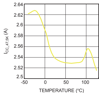
CC Charge Current vs. Temperature R_{ISET}=47.5k\Omega
