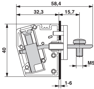
Dimensioned drawing
