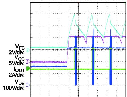
OLP Power-On
