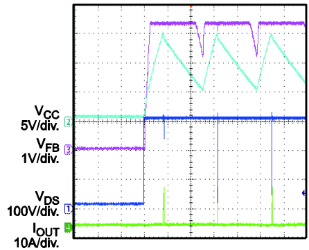
SCP Power-On
