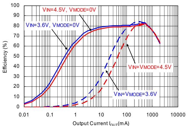
RP506Lxx1K/L/M V_{OUT} = 1.2\text{ V}
