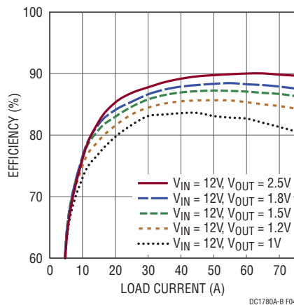
Figure 4. Measured Efficiency V IN = 12V, f SW = 500kHz
