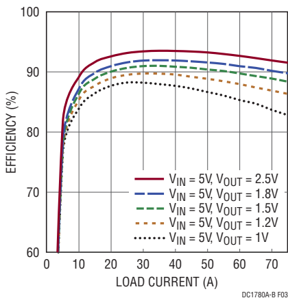
Figure 3. Measured Efficiency V IN = 5V, f SW = 500kHz
