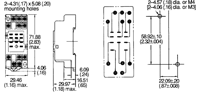
Terminal arrangement/ mounting holes (Top view)
