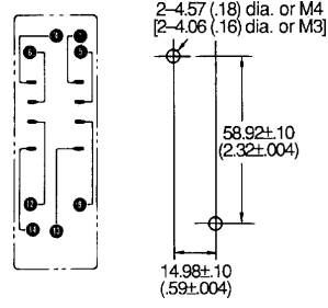
Terminal arrangement/ mounting holes (Top view)
