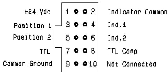
Switch connector
