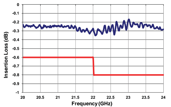
Insertion Loss (20-24 GHz)
