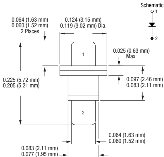
Dimensions are in inches (millimeters shown in parentheses) 203235-006
