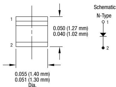
Dimensions are in inches (millimeters shown in parentheses) 203235-005
