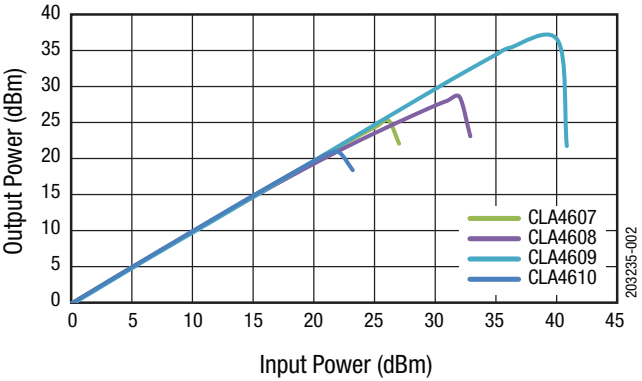
Figure 2. CLA4607 to CLA4610 CW Output vs Input Power
