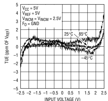
Total Unadjusted Error ( V_{CC} = 5V , V_{REF} = 5V )
