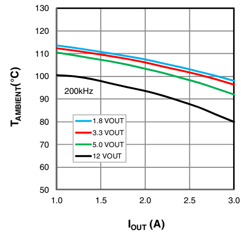
Figure 30: XR76203, V_{IN}=24\text{V}
